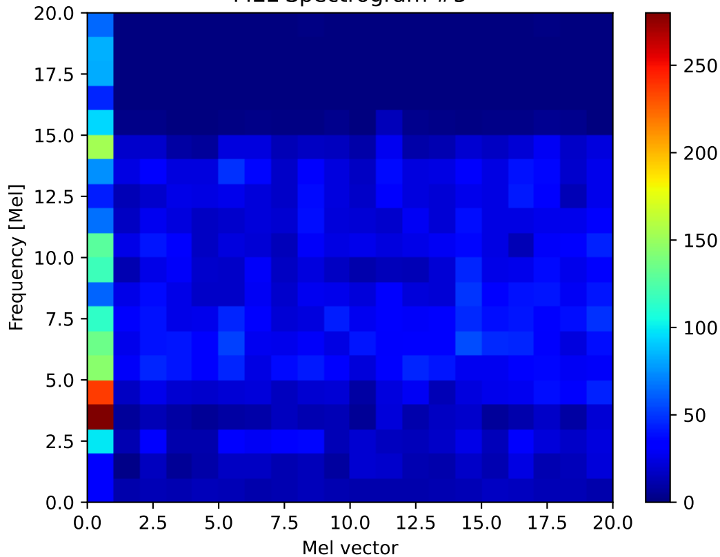
MEL Spectrogram #5
